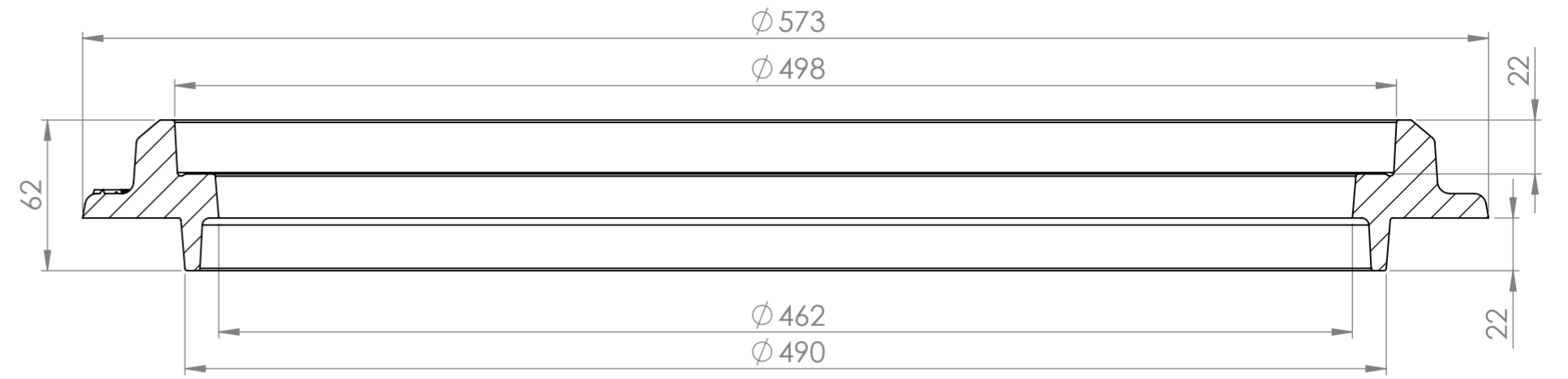
SECTION A-A SCALE 1 : 2.5
