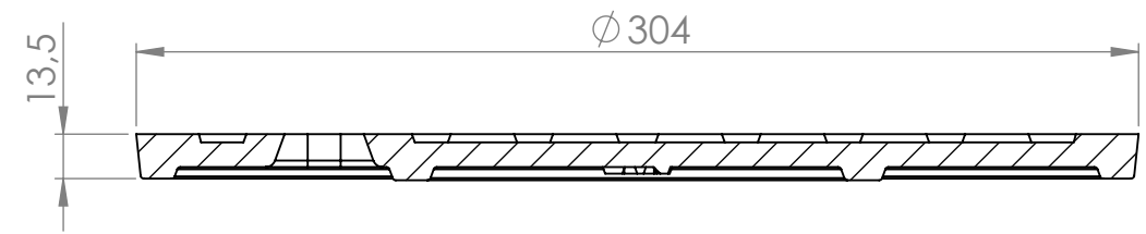
SECTION A-A SCALE 1 : 2.5
