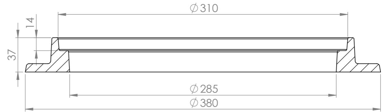
SECTION A-A SCALE 1 : 2.5
