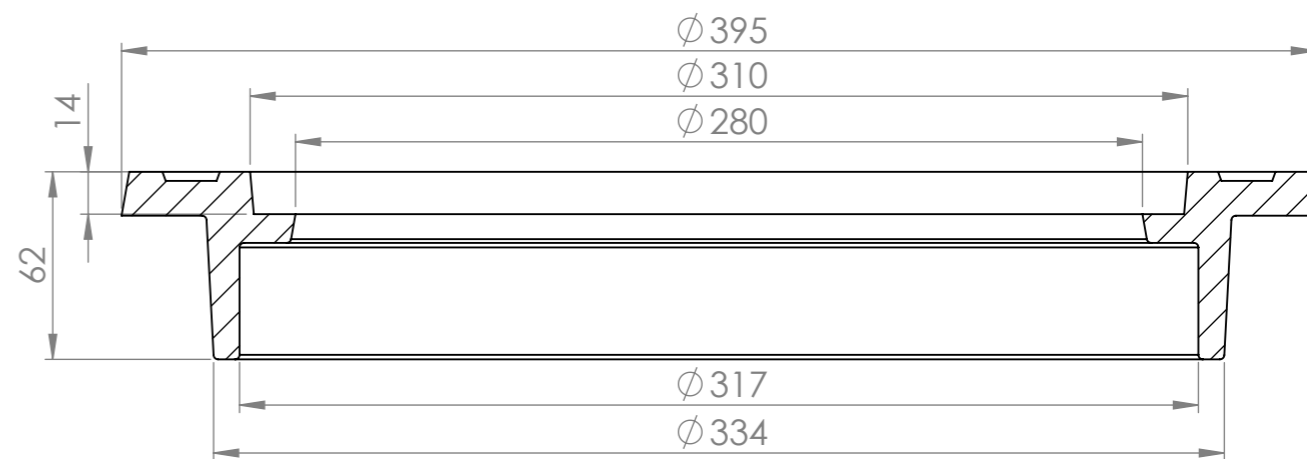
SECTION A-A SCALE 1 : 2.5
