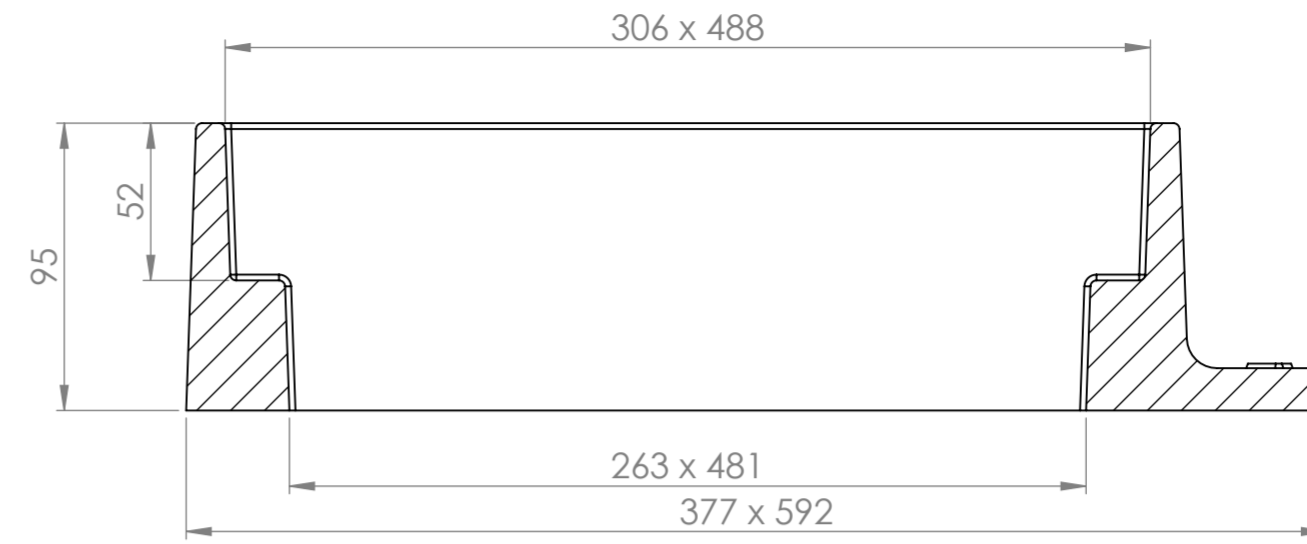
SECTION A-A SCALE 1 : 2.5
