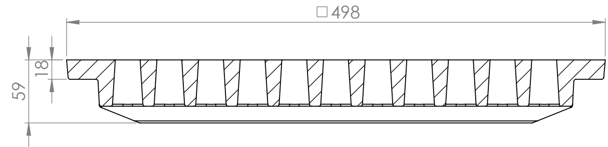
SECTION A-A SCALE 1 : 3.5
