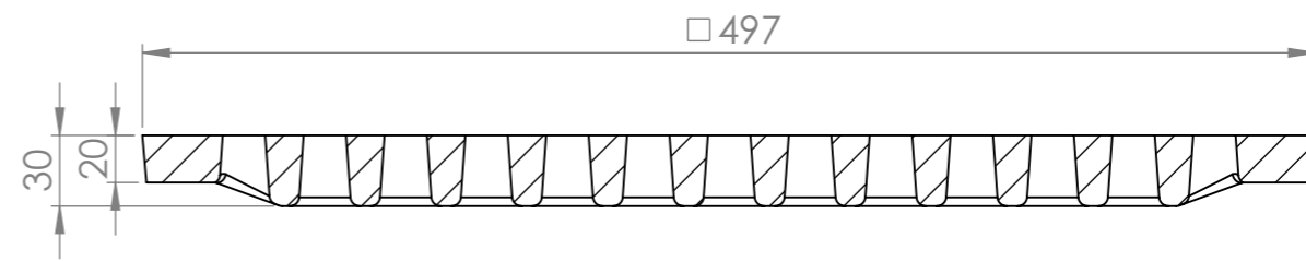
SECTION A-A SCALE 1 : 3.5
