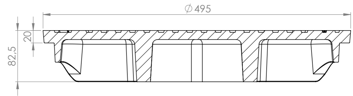
SECTION A-A SCALE 1 : 3.5
