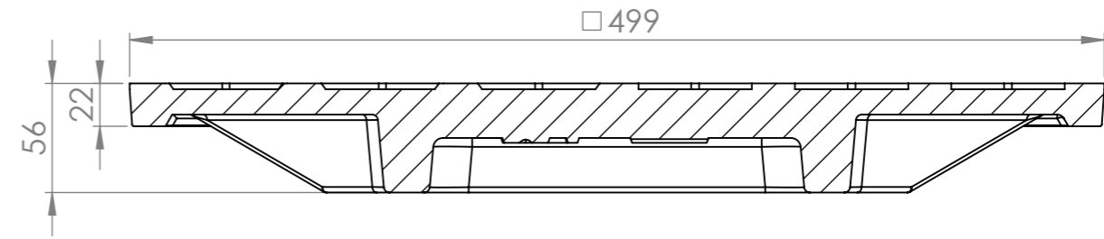
SECTION A-A SCALE 1 : 3.5
