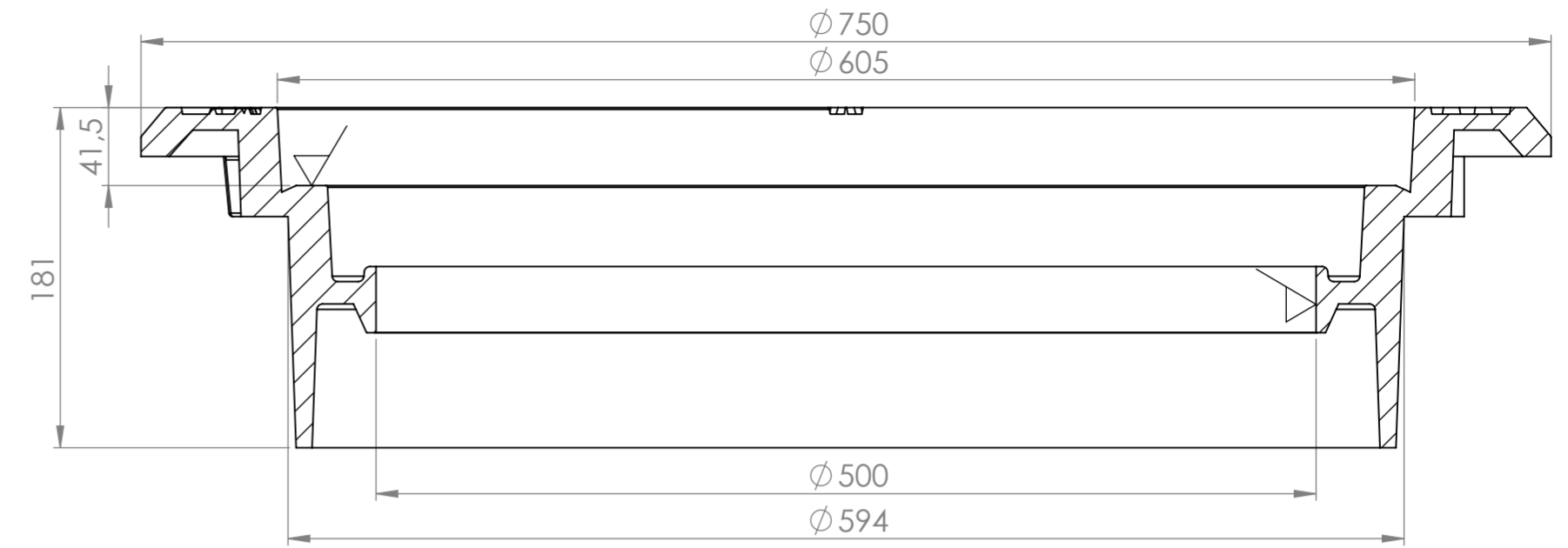
SECTION A-A SCALE 1 : 3.5
