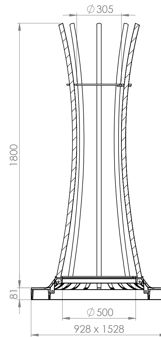
SECTION C-C
